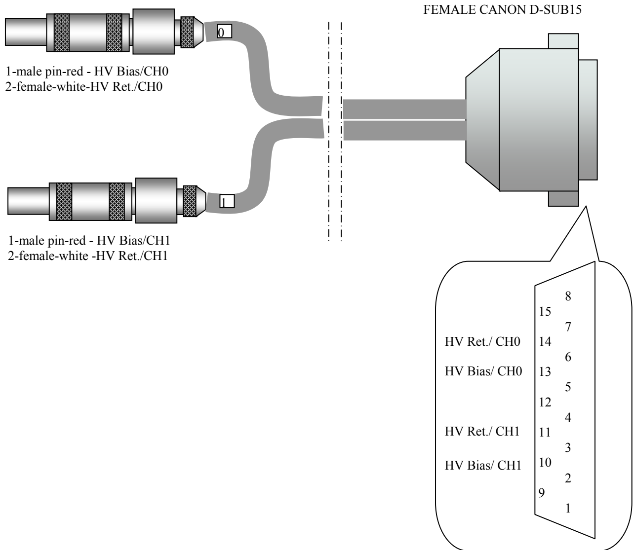
Figure 6. LV-HV interconnection cable
